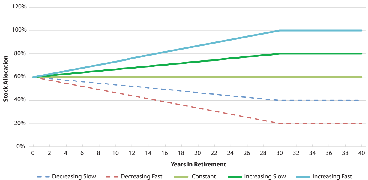
Figure 1: Glide Paths Showing Stock Allocation over Time Assuming a 60% Initial Stock Level
