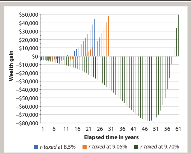
Figure 1: Breakeven Time for Three r -taxed Rates
