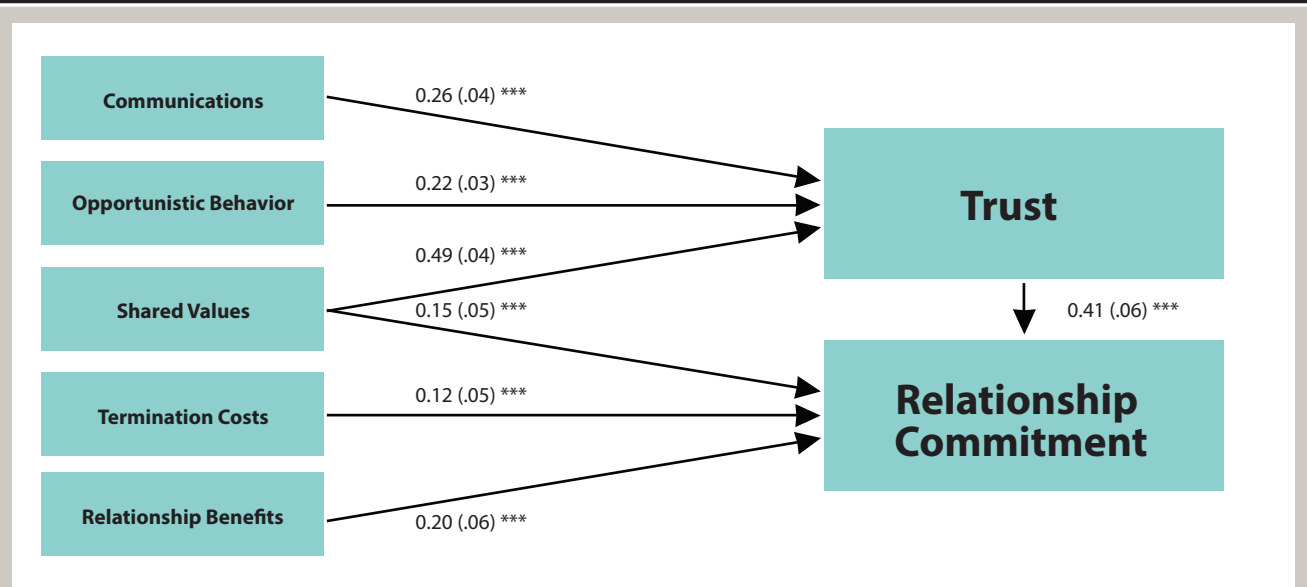
Figure 1: Path Diagram with Standardized Coefficients (Standard Errors)
