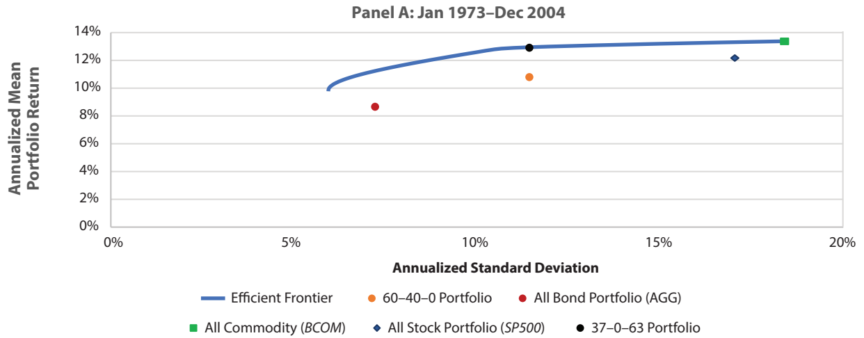
Figure 2: Efficient Frontier
