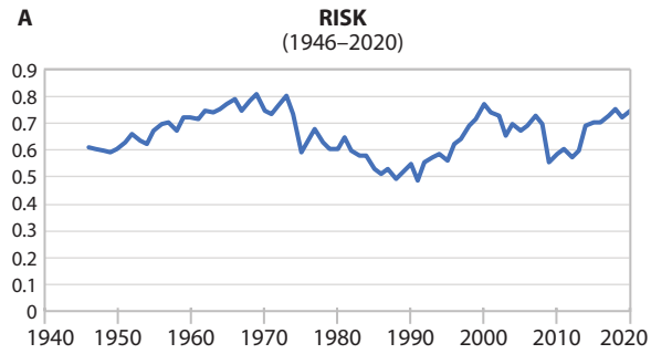
Figure 1: A Time-Series Plot of RISK and CAPE
